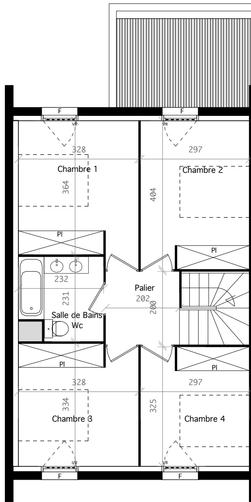
Plan R+1
