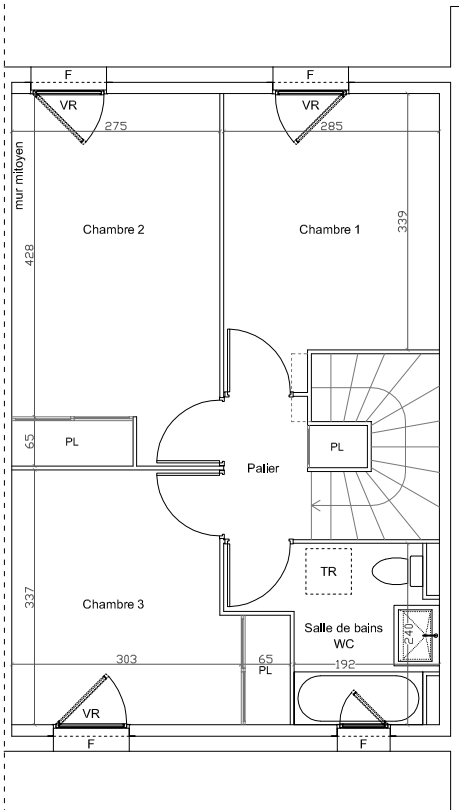
Plan R+1
